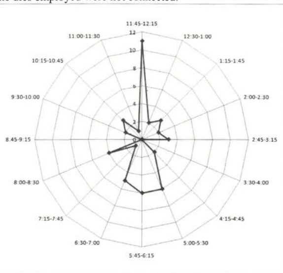
Radar chart 1. Die axis indices of the Georgian-Hulagid Christian dirhams from the Dikhashkho hoard.
